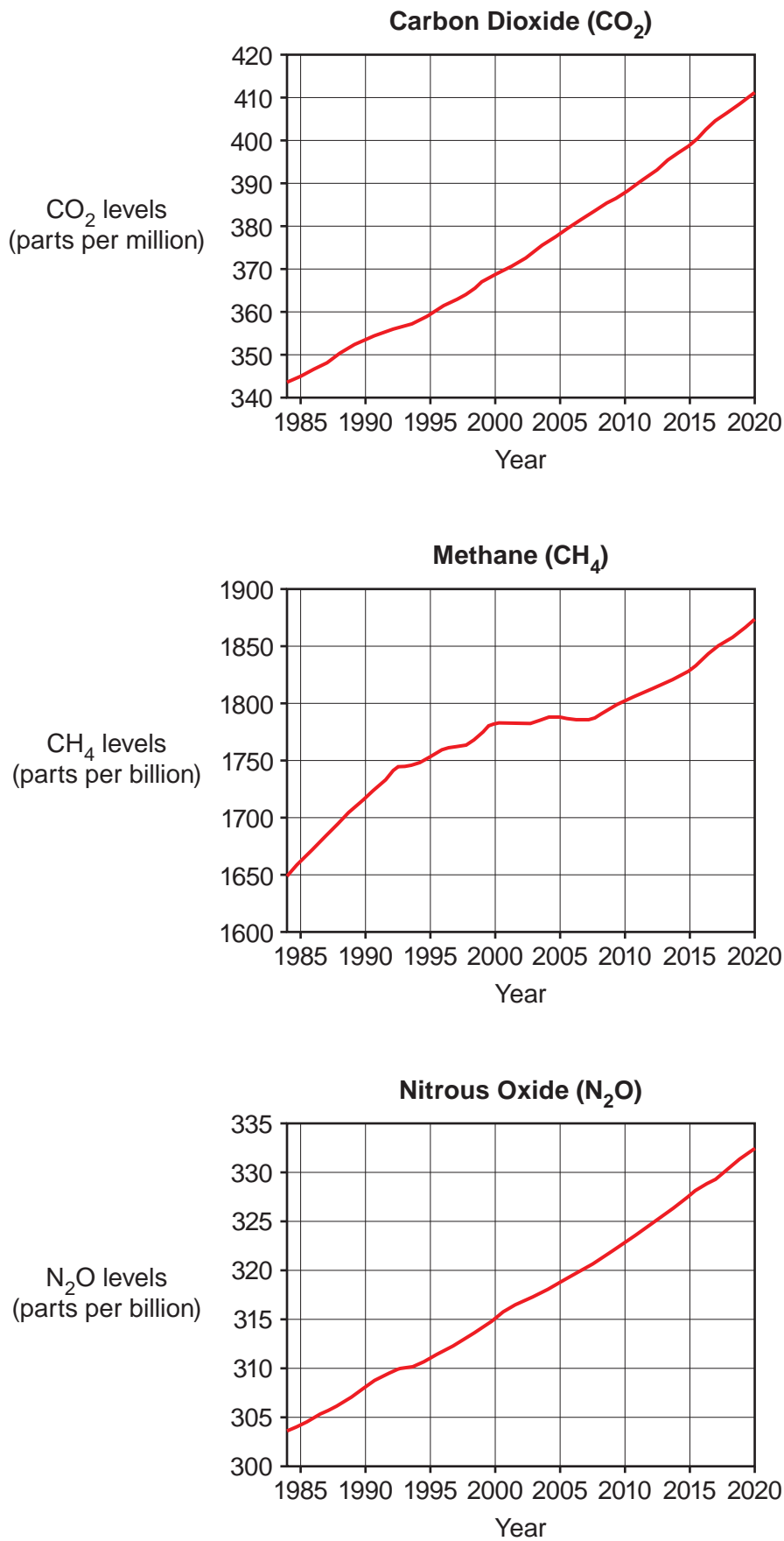
Fig. 3 Changes in greenhouse gas levels from 1985 to 2020
